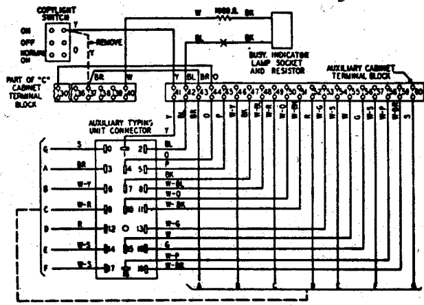
MODIFICATION OF WIRING OF 28 TTY CABINET USING PARTS FURNISHED WITH 28 TYPE TYPING UNITS
