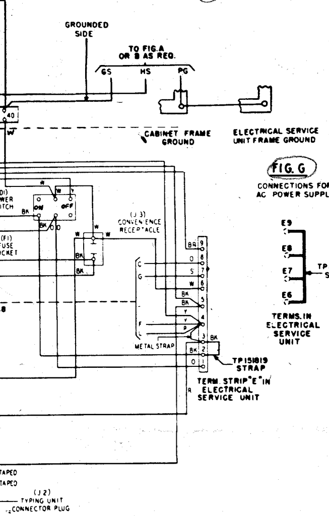
MODIFICATION OF WIRING OF 28 TTY CABINET USING PARTS FURNISHED WITH 28 TYPE TYPING UNITS
