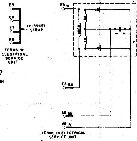
FIG. G CONNECTIONS FOR AC POWER SUPPLY
