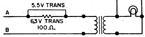
FIG. C 6V COPY LAMPS WITH TRANSFORMER
