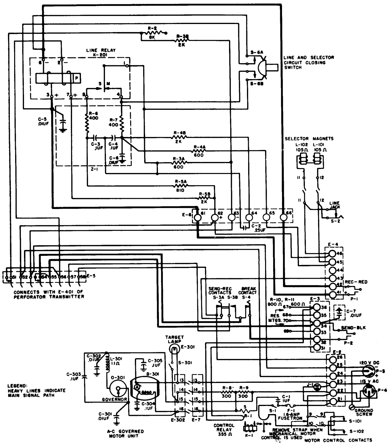
Figure 268. Typing unit, base and relay, schematic wiring diagram.
